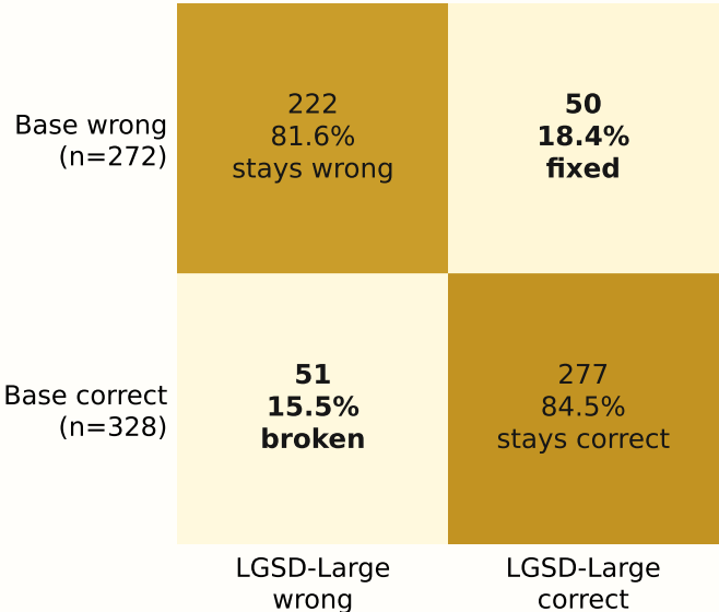
LGSD-Large: 50 fixed, 51 broken (net -1)
