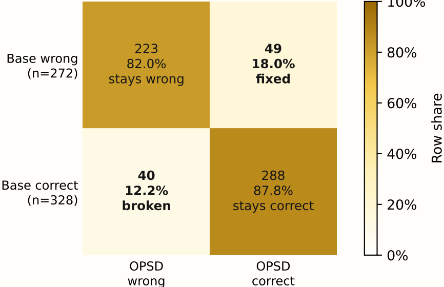
OPSD: 49 fixed, 40 broken (net +9)
