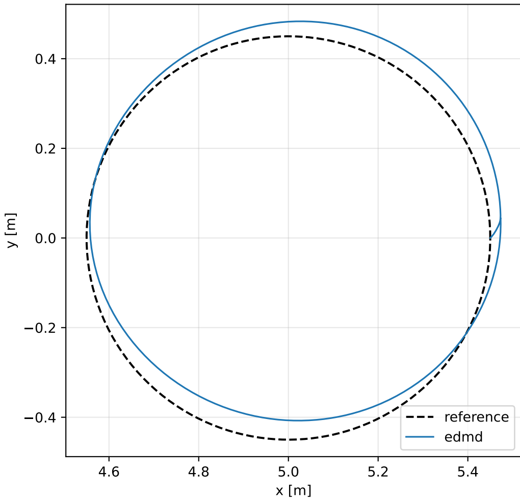
End-effector path
