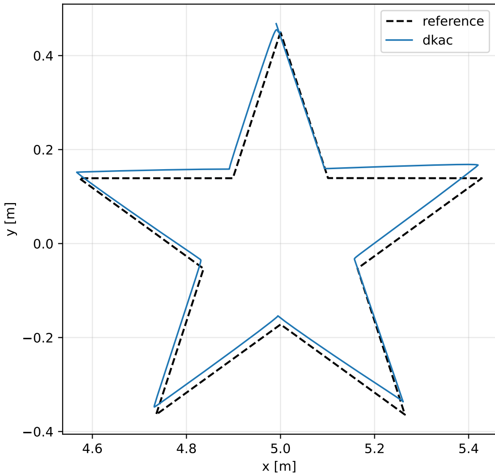
End-effector path
