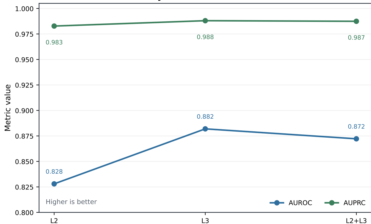
PatchCore layer ablation: detection metrics
