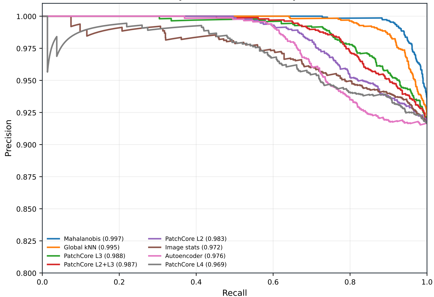
Overall precision-recall comparison
