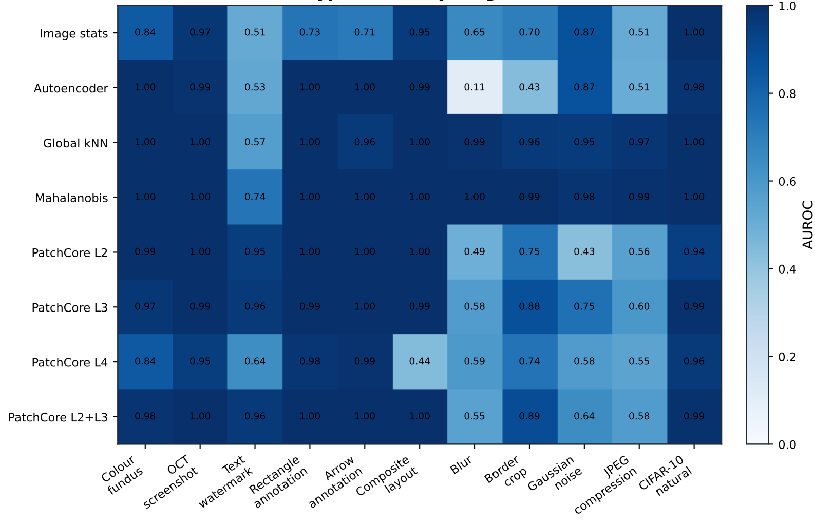
Per-subtype AUROC by Stage 1 method
