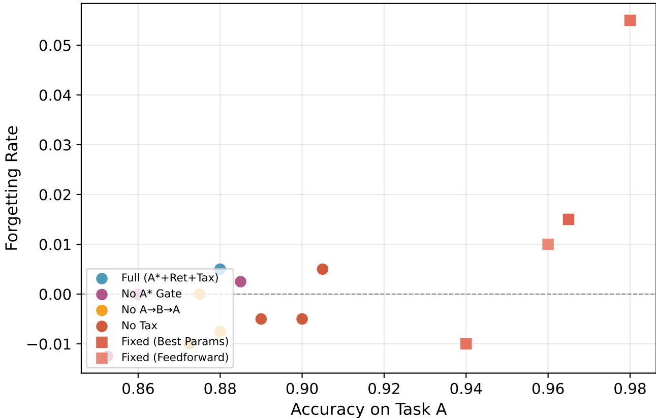
Figure 2: Accuracy vs Forgetting Trade-off (Evolving: circles, Fixed: squares)
