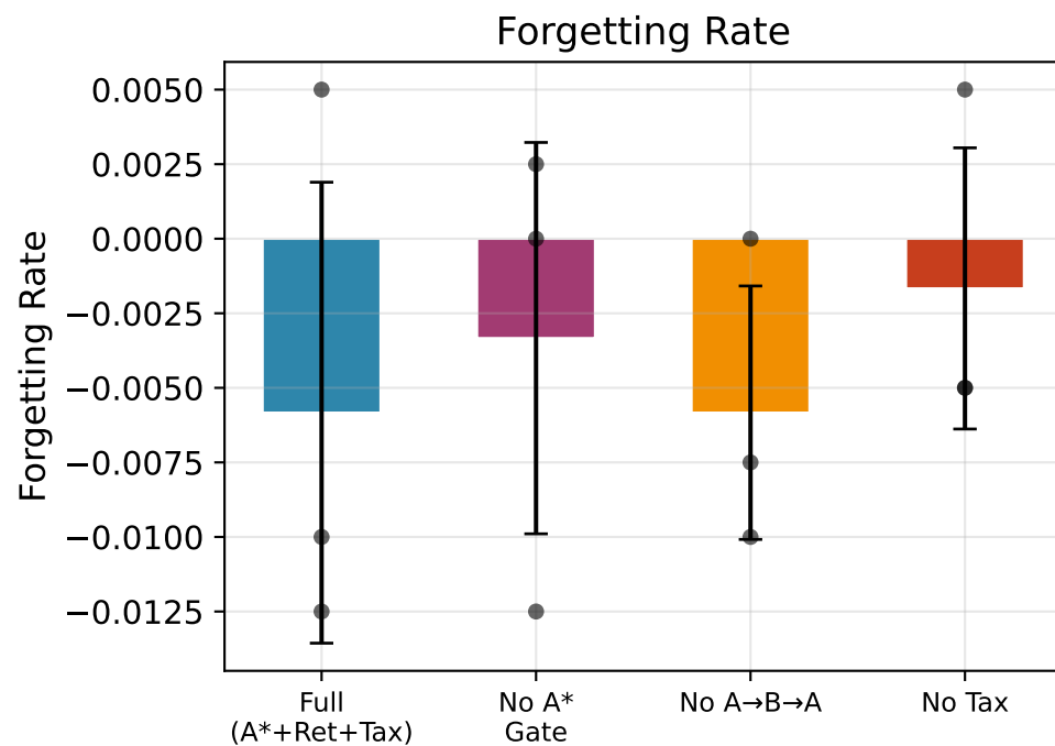
Figure 3: Ablation Analysis — Effect of Removing Components (4 evolving configs \times 3 seeds)
