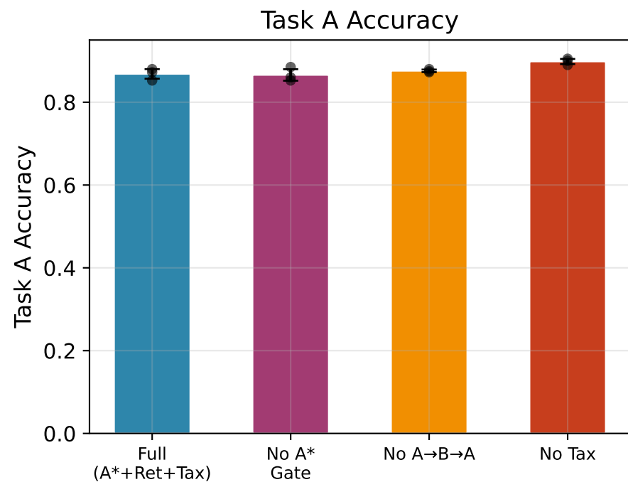
Figure 3: Ablation Analysis — Effect of Removing Components (4 evolving configs \times 3 seeds)
