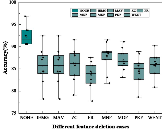
Fig. 4. Accuracy distribution for different feature deletion cases.
