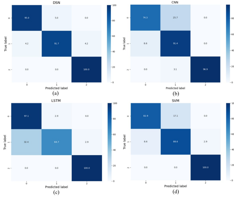
Fig. 3. Confusion matrix for 4 models
