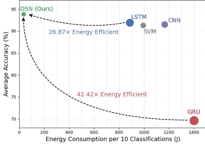
Fig. 1. Energy Consumption vs. Average Accuracy for Different Models.
