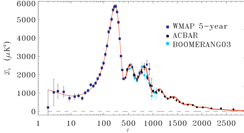
Figure 17: Anisotropy of CMB temperature.
