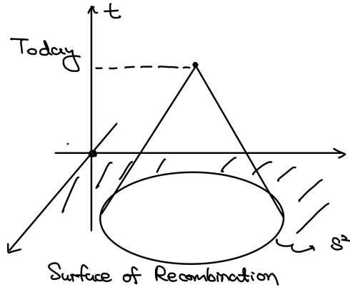
Figure 18: Propagation of CMB photons.
