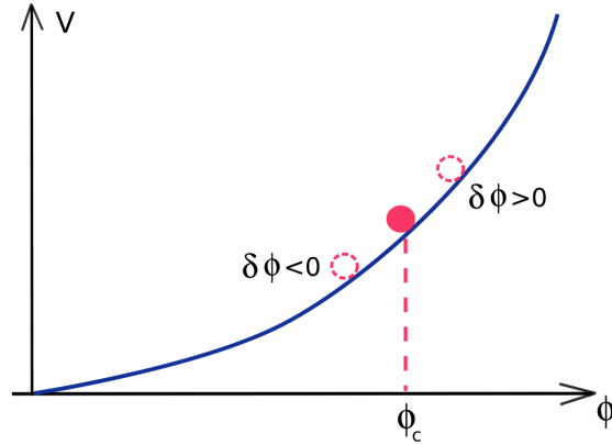
Figure 25: The end of inflation
