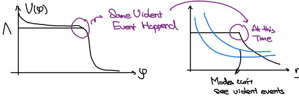
Figure 24: The potential of the inflaton field.
