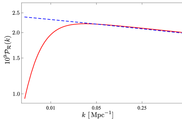
Figure 20: Primordial Power Spectrum, here \mathcal{P} is the dimensionless power spectrum defined as \mathcal{P} \sim k^3 P
