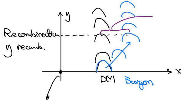
Figure 16: The oscillation of baryon and radiation fluid, and the static dark matter perturbation.
