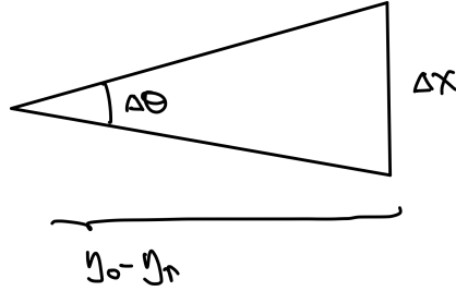
Figure 19: The relation between the physical distance and the angle.
