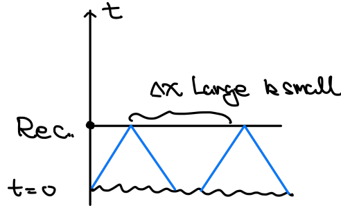
Figure 20: The horizon problem
