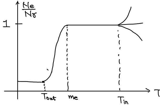
Figure 9: The plot of the number density of electrons as a function of temperature.
