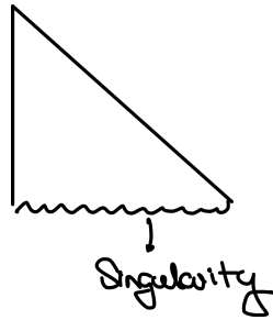
Figure 1: Penrose diagram for a decelerating universe with \omega > -\frac{1}{3}
