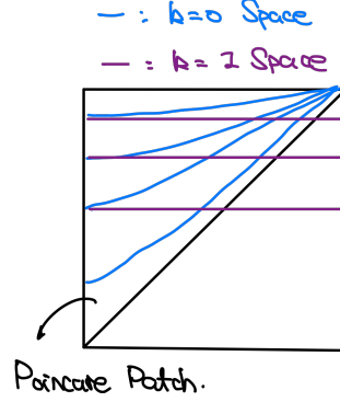
Figure 5: Penrose diagram for the global dS spacetime, where the blue region is the Poincare patch which is the cosmological constant case with flat spatial curvature
