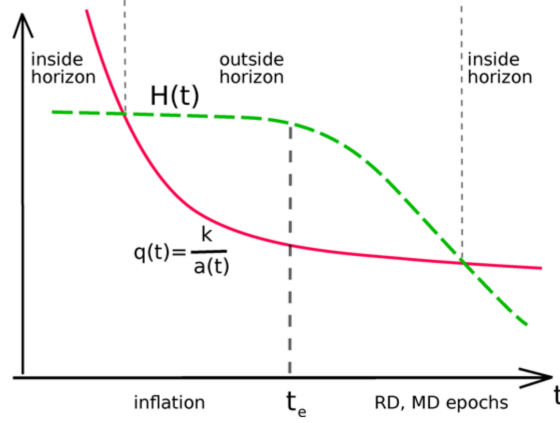
Figure 22: Illustration of solving Horizon Problem with dS.
