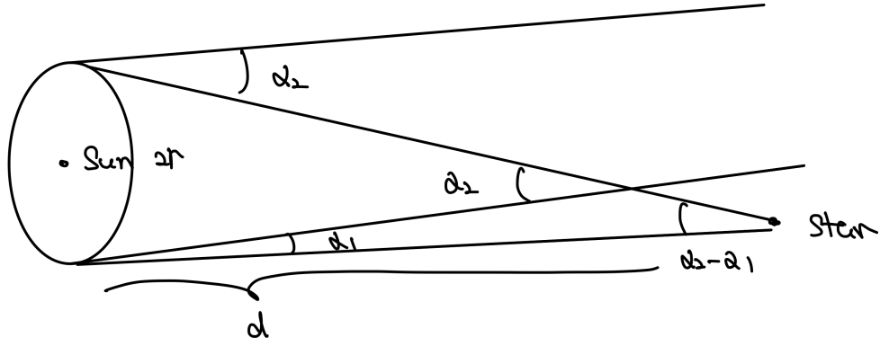
Figure 6: Parallax measurement.
