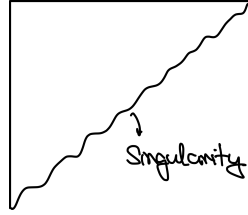
Figure 4: Penrose diagram for cosmological constant case with \omega < -1
