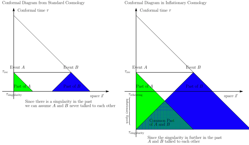
Figure 21: The history of the universe in the inflation theory.
