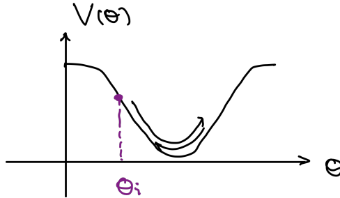
Figure 14: The axion field starts to oscillate.
