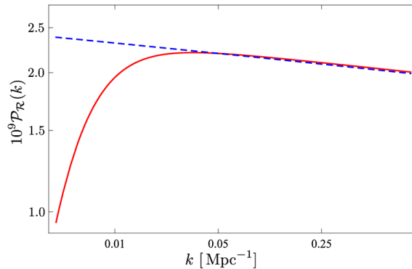
Figure 19: Primordial Power Spectrum, here \mathcal{P} is the dimensionless power spectrum defined as \mathcal{P} \sim k^3 P
