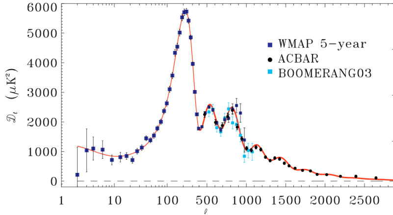
Figure 16: Anisotropy of CMB temperature.
