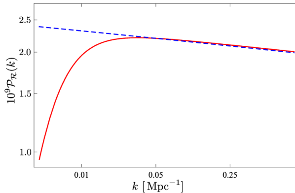
Figure 19: Primordial Power Spectrum, here \mathcal{P} is the dimensionless power spectrum defined as \mathcal{P} \sim k^3 P
