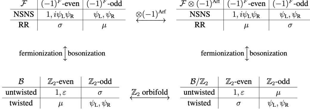
Figure 1: Duality web relating Ising CFT and Majorana CFT.
