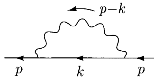
Figure 2: First order correction to the fermion propagator in QED.
