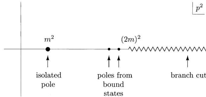
Figure 1: The isolated pole of the correlation function is a particle
