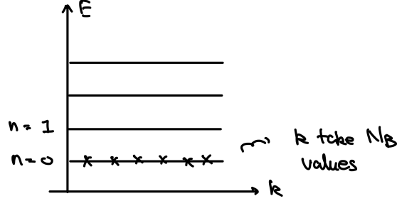
Figure 2: Landau levels
