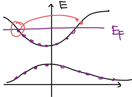
Figure 1: Band structure
