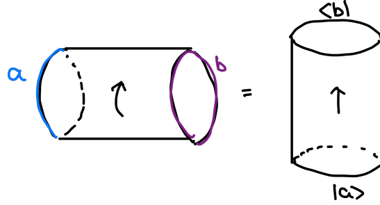
Figure 3: Cardy's condition of possible boundary conditions.
