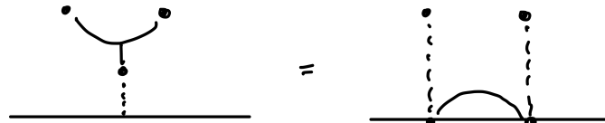
Figure 7: Bulk-Bulk Sewing Constraint.
