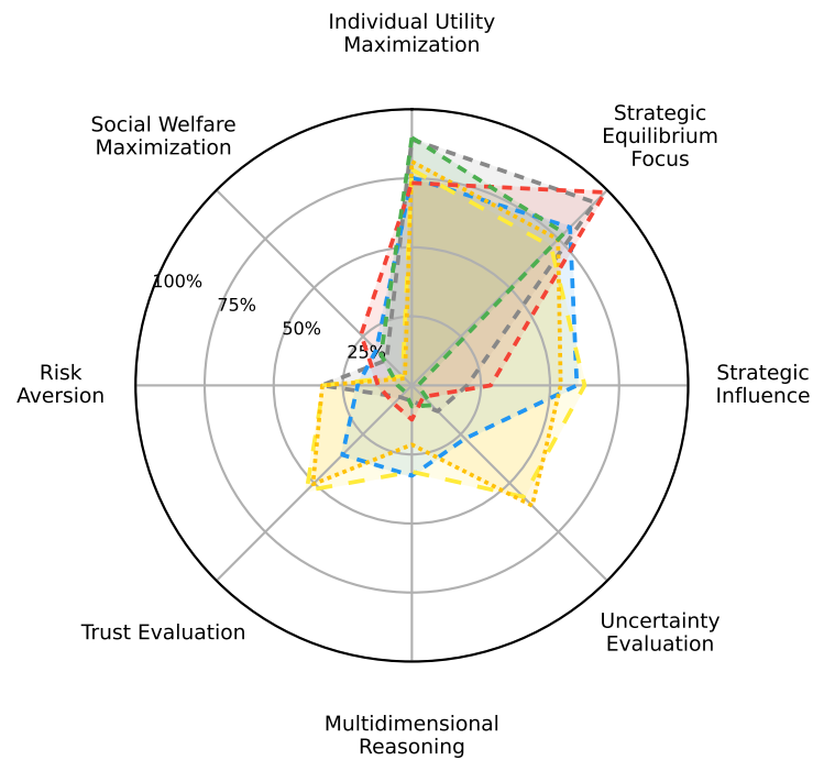
Justification by Gemini-R
