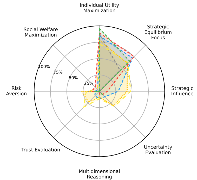
Justification by GPT-5.2
