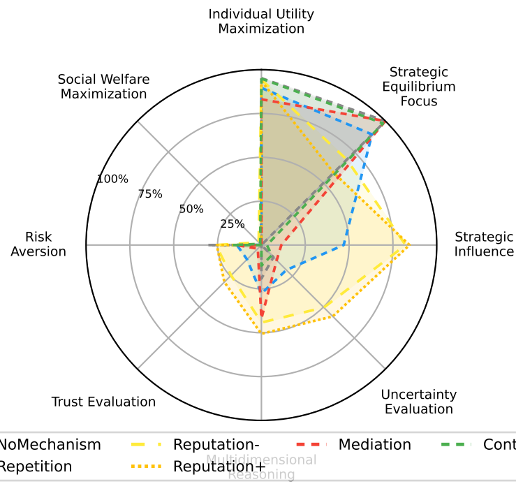
Justification by Qwen-30b
