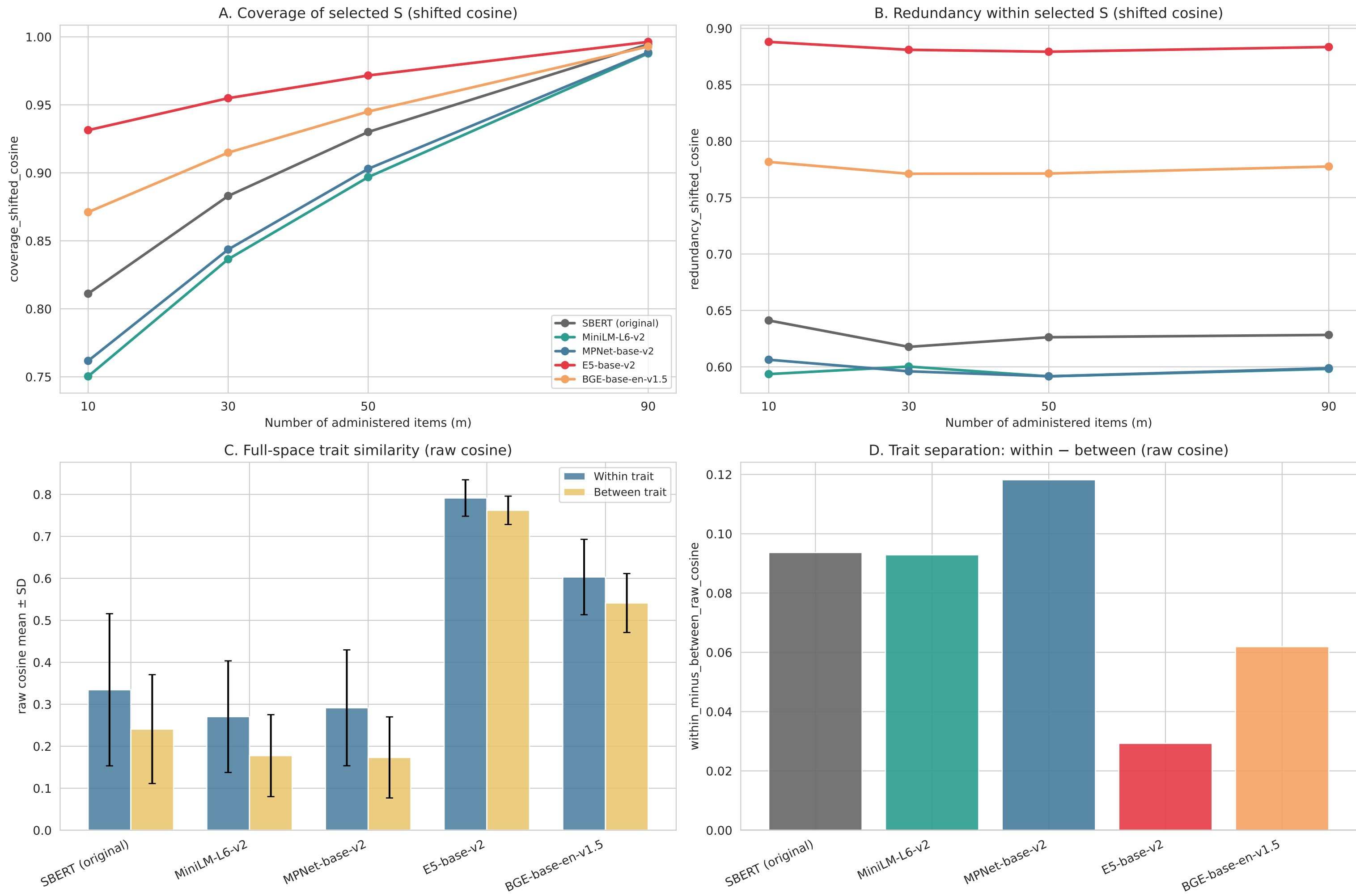
Figure 5: Embedding Space Quality Diagnostics
