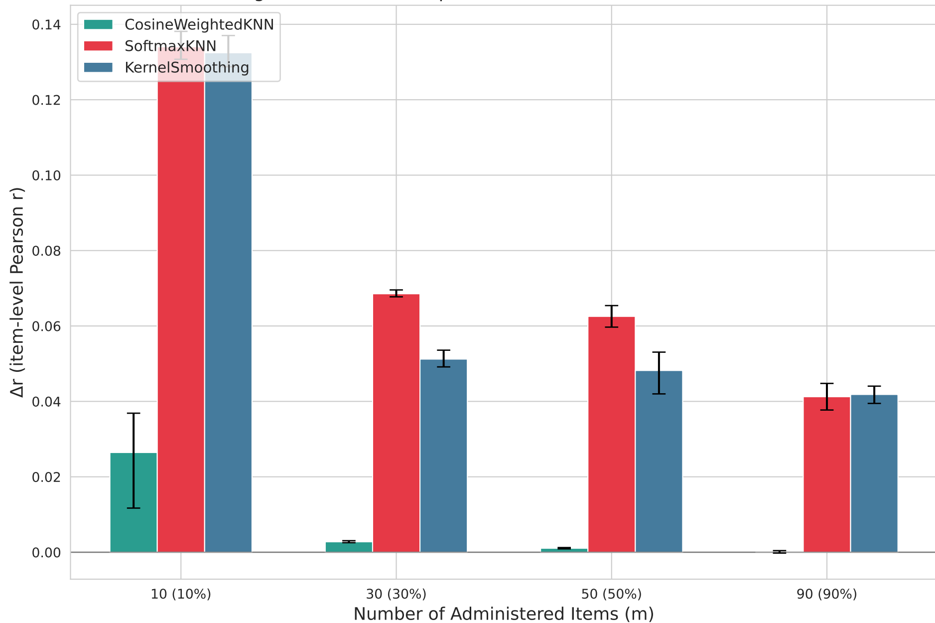
Figure 3: Predictor Improvement over Tuned UniformKNN
