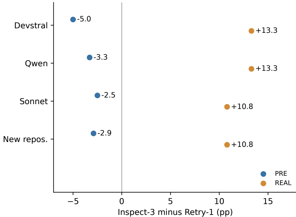
(a) Protocol-specific policy advantage
