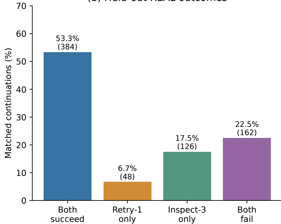
(b) Held-out REAL outcomes
