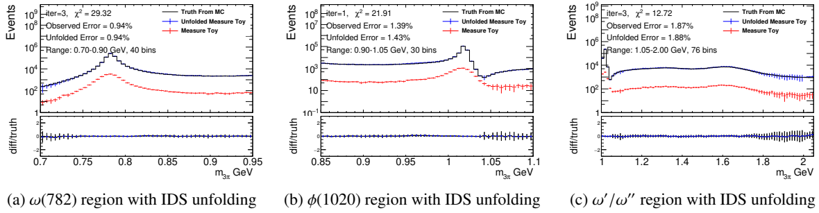
Figure 13: Unfolded results for three representative mass regions using the IDS method with optimized parameters. Each panel shows the true MC distribution (black), the measured MC distribution (red), and the unfolded result (blue points) with its statistical uncertainties. The MC sample has been normalized to match the data statistics shown in Fig. 11, ensuring that the uncertainties properly reflect the data statistical power.
