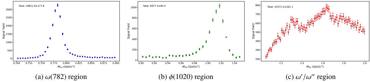
Figure 21: Extracted signal yields as a function of M_{3\pi} after applying helix parameter corrections to the signal MC and the \chi_{4C}^2 < 50 selection requirement. The three mass regions are shown separately. The error bars represent the statistical uncertainties from the fits. The \omega(782) and \phi(1020) resonances appear as clear peaks, while the higher-mass region reveals broader structures corresponding to excited \omega states.
