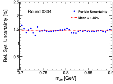
(a) Round 03/04, \omega(782) region
