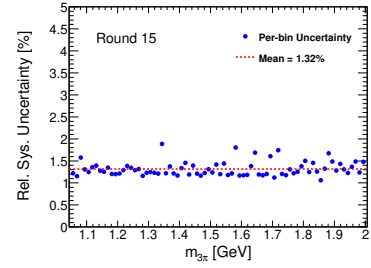
(f) Round 15, \omega'/\omega'' region
