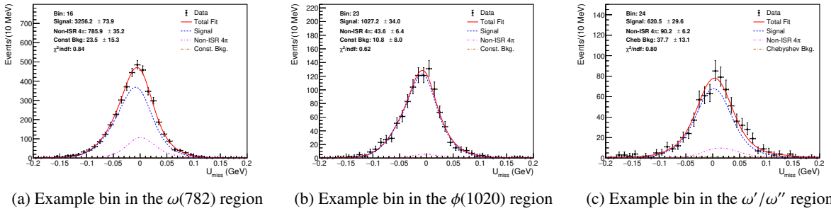
Figure 10: Typical U_{\text{miss}} fit results for representative M_{3\pi} bins from each of the three mass regions.
