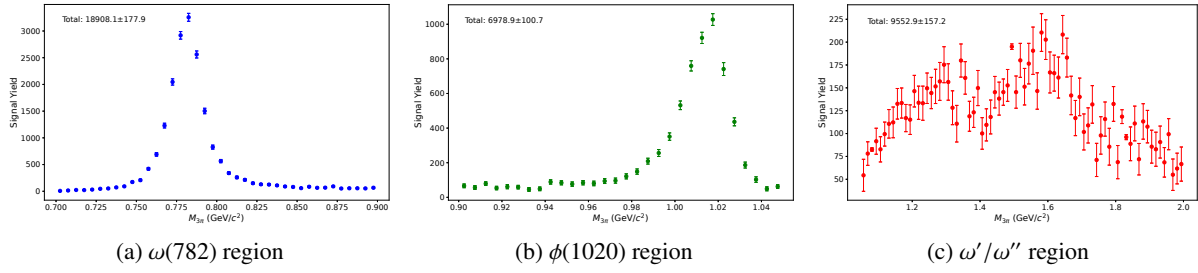
Figure 11: Extracted signal yields as a function of M_{3\pi} for the three mass regions. The error bars represent the statistical uncertainties from the fits. The \omega(782) and \phi(1020) resonances appear as clear peaks, while the higher-mass region reveals broader structures corresponding to excited \omega states.
