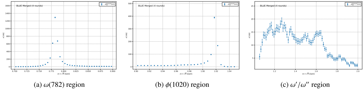
Figure 24: BLUE-combined dressed cross section \sigma_{3\pi}^{\text{dress}}(m) results for the three invariant mass regions. The error bars represent the statistical uncertainties propagated from the covariance matrices. The combination significantly improves the statistical precision compared to any single data-taking period.
