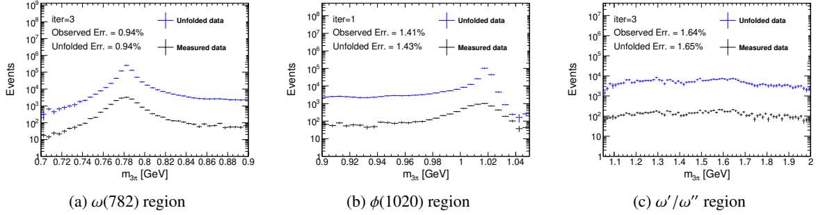
Figure 22: Unfolded M_{3\pi} distributions for data after applying the corrected response matrix. The results are shown only within the nominal mass ranges defined in Tab. 4.
