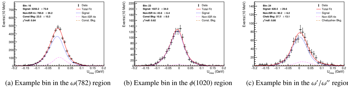
Figure 9: Typical U_{\text{miss}} fit results for representative M_{3\pi} bins from each of the three mass regions.
