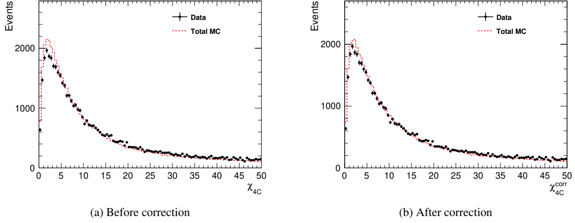
Figure 20: Comparison of \chi^2_{4C} distributions between data and MC for the e^+e^- \rightarrow \pi^+\pi^-\pi^0\gamma_{\text{ISR}} process (a) before and (b) after applying helix parameter corrections.
