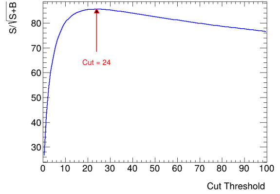
(b) FOM scan as a function of the \chi^2 cut
