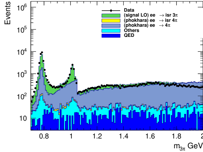
Figure 4: The 3\pi invariant mass distribution after applying the \chi_{\text{KF}}^2 < 24 selection. The stacked histogram shows the contributions from the signal process e^+e^- \rightarrow \pi^+\pi^-\pi^0 and various background processes, including the dominant e^+e^- \rightarrow \pi^+\pi^-\pi^0\pi^0 and e^+e^- \rightarrow \pi^+\pi^-\pi^0\pi^0\gamma_{\text{ISR}} backgrounds.
