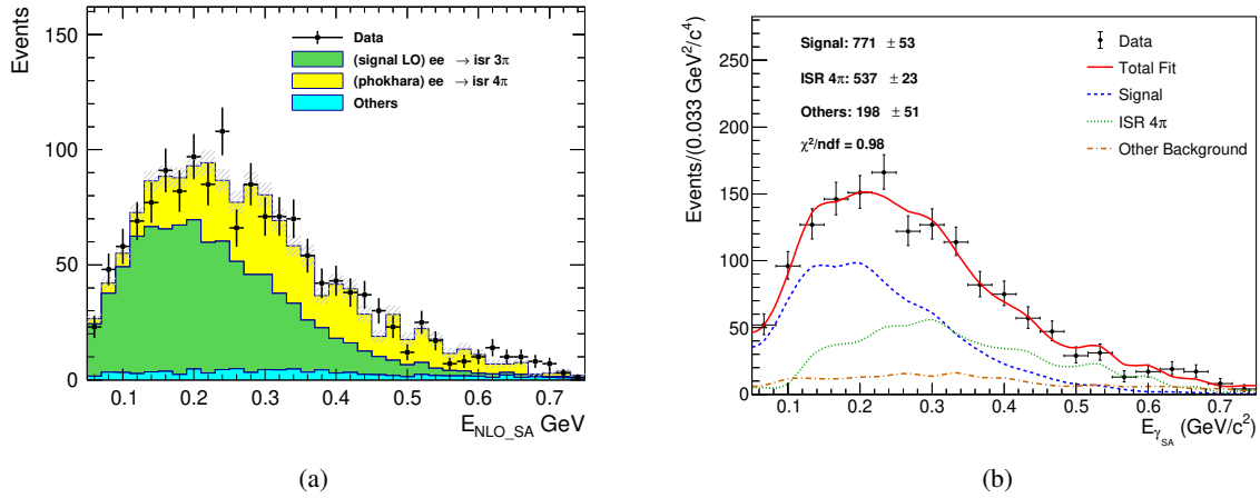
Figure 20: (a) Laboratory energy distribution of the inferred SA photon candidate. (b) Fit to the distribution.
