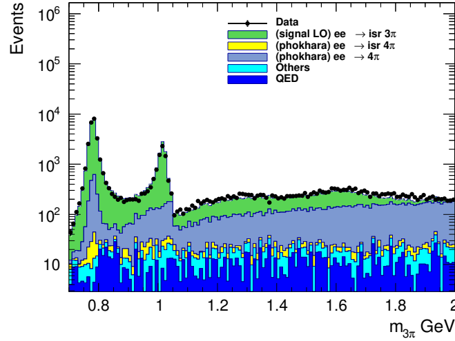
Figure 4: The 3\pi invariant mass distribution after applying the \chi^2_{\text{KF}} < 50 selection to the Round 16 data sample. The stacked histogram shows the contributions from the signal process e^+e^- \rightarrow \pi^+\pi^-\pi^0 and various background processes, including the dominant e^+e^- \rightarrow \pi^+\pi^-\pi^0\pi^0 and e^+e^- \rightarrow \pi^+\pi^-\pi^0\pi^0\gamma_{\text{ISR}} backgrounds.
