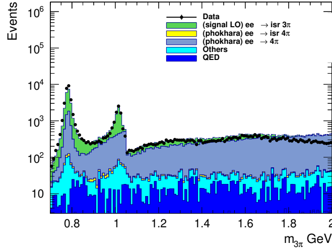
Figure 3: The 3\pi invariant mass distribution after applying the \chi^2_{\text{KF}} < 24 selection. The stacked histogram shows the contributions from the signal process e^+e^- \rightarrow \pi^+\pi^-\pi^0 and various background processes, including the dominant e^+e^- \rightarrow \pi^+\pi^-\pi^0\pi^0 and e^+e^- \rightarrow \pi^+\pi^-\pi^0\pi^0\gamma_{\text{ISR}} backgrounds.
