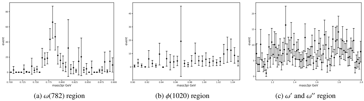
Figure 8: Estimated background contributions from e^+e^- \rightarrow \gamma_{\text{ISR}}\pi^+\pi^-\pi^0\pi^0 in the signal region after scaling, using data from round 16. The three panels correspond to different 3\pi invariant mass regions: (a) the \omega(782) region, (b) the \phi(1020) region, and (c) the higher-mass \omega'/\omega'' region.
