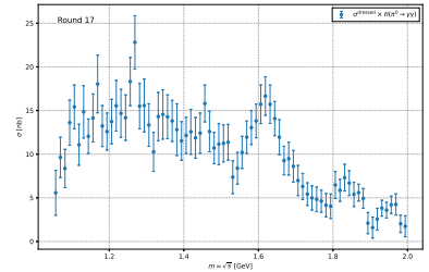
(l) Round 17, \omega'/\omega'' region
