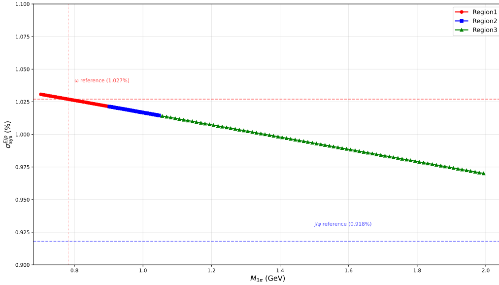
Figure 24: Systematic uncertainties from the E/p requirement, obtained from linear interpolation between \omega and J/\psi using \sigma_{\text{sys}} = |\delta| + |\sigma_\delta| .
