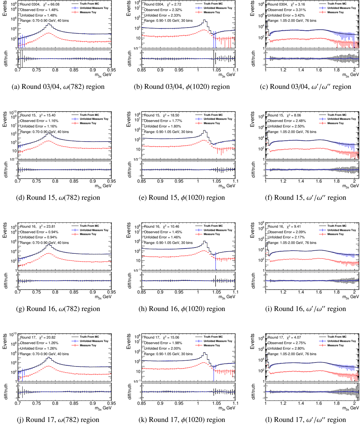
Figure 20: Unfolded results for four data-taking periods (Round 03/04, Round 15, Round 16, Round 17) using the IDS method. The unfolding parameters were optimized using the Round 16 MC sample (third row) and then applied to all rounds.
