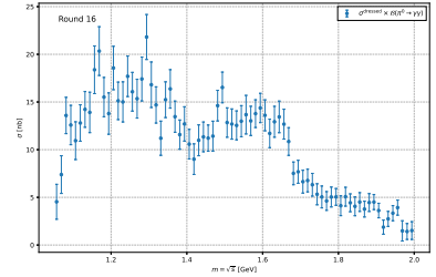
(i) Round 16, \omega'/\omega'' region
