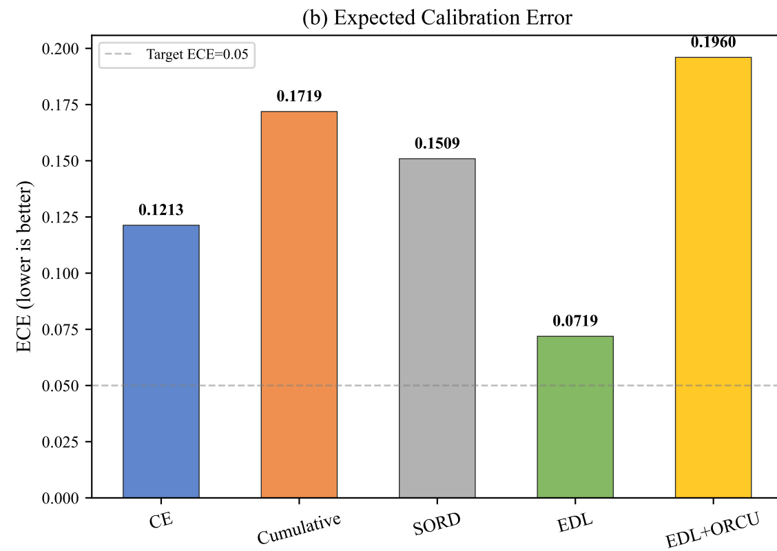
Figure 5: Mode Comparison — DF Fluorosis (v2.2, ViT-Base)
