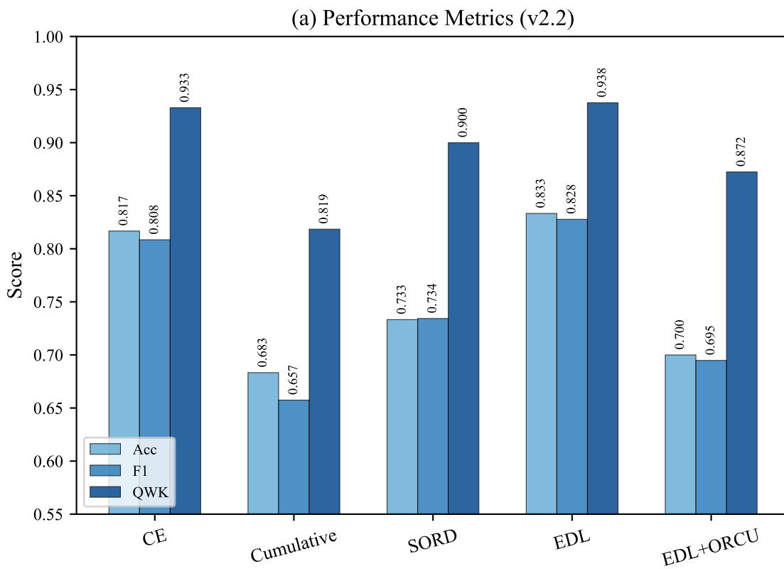
Figure 5: Mode Comparison — DF Fluorosis (v2.2, ViT-Base)
