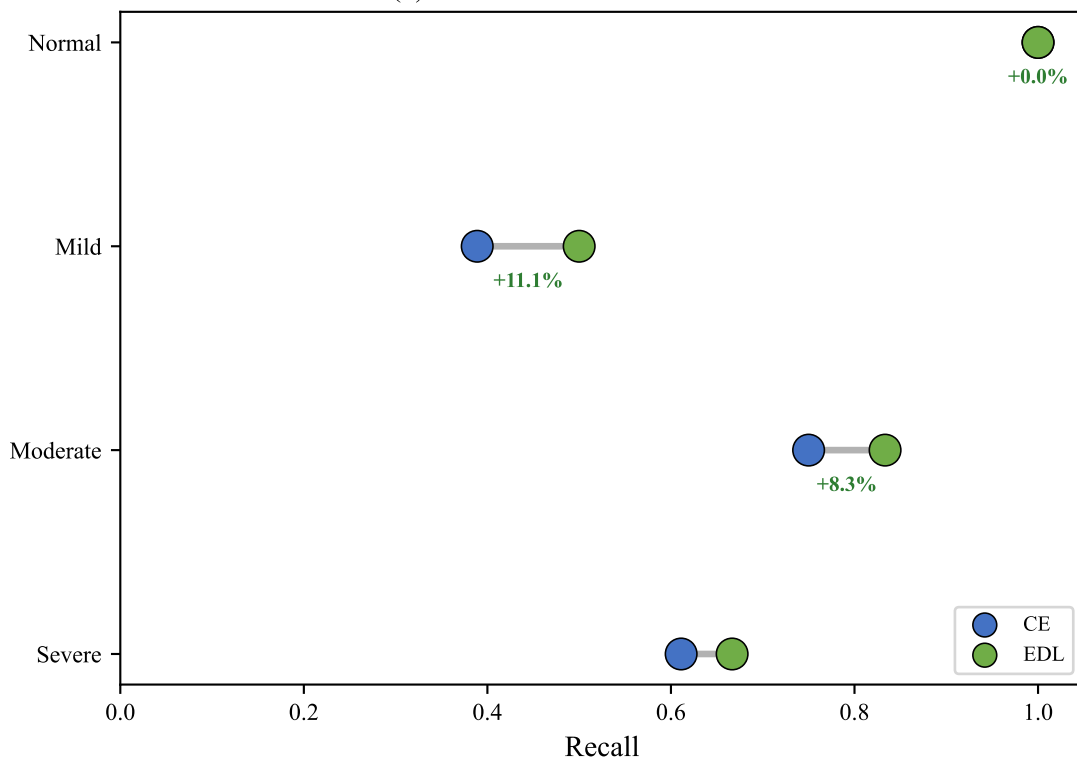
(c) Per-Class Recall: CE \rightarrow EDL
