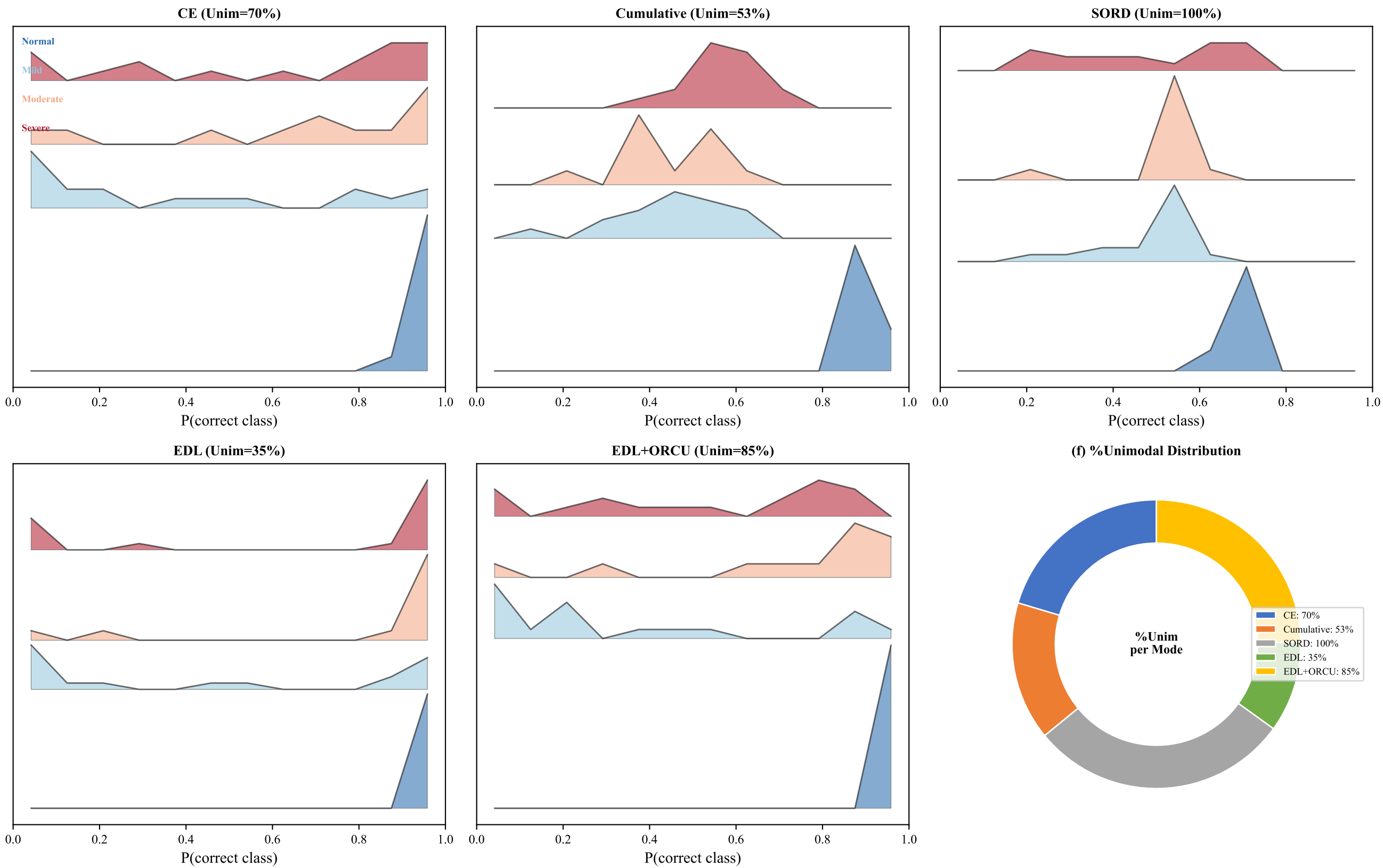
Figure 8: Prediction Probability Distribution & Unimodal Pattern
