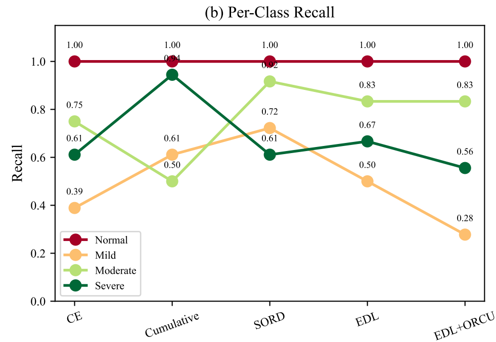
Figure 10: Per-Class Performance Analysis
