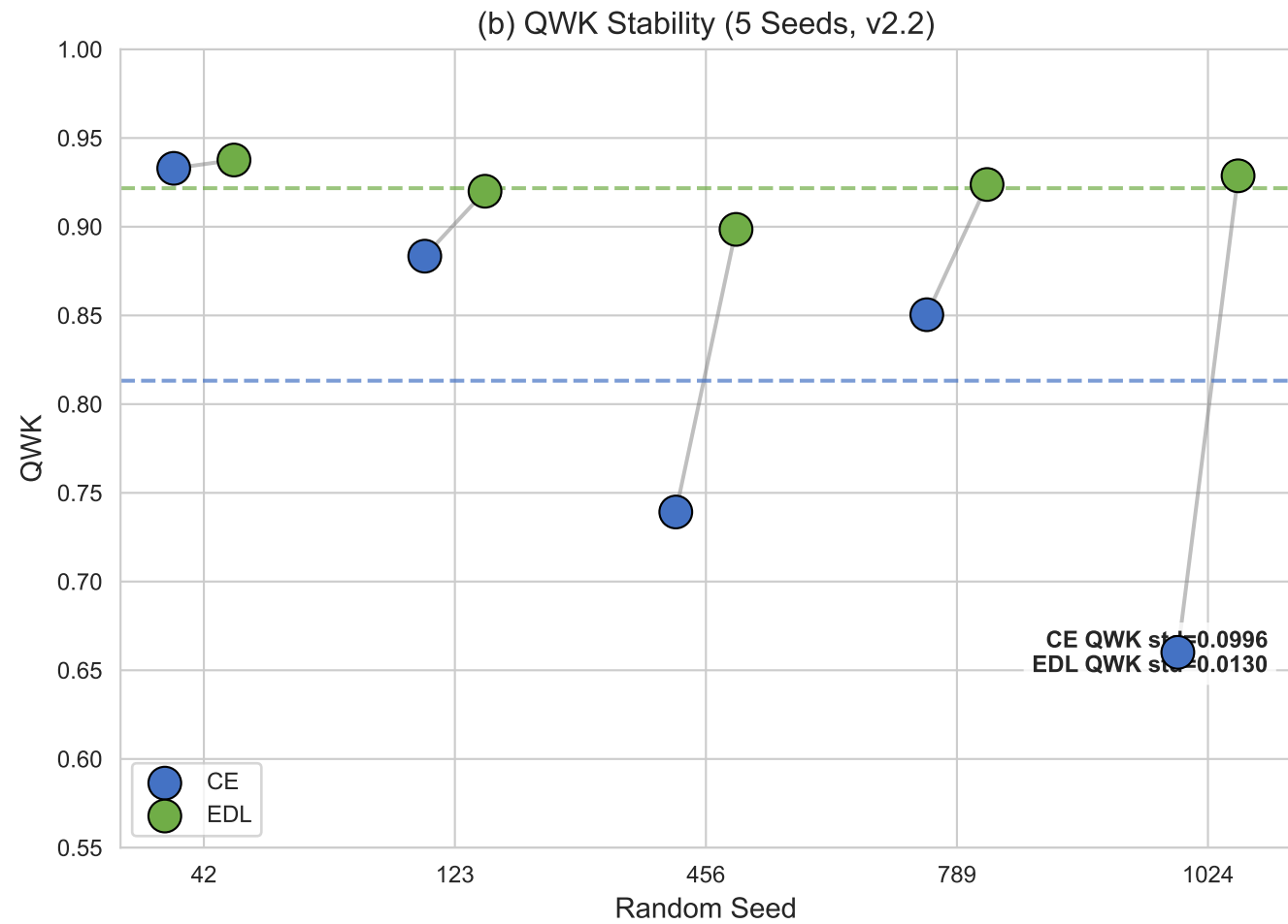
Figure 12: Training Stability — CE vs EDL (ViT-Base, DFID)
