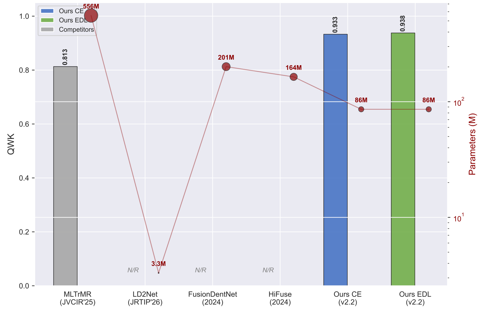
(b) QWK & Model Complexity
