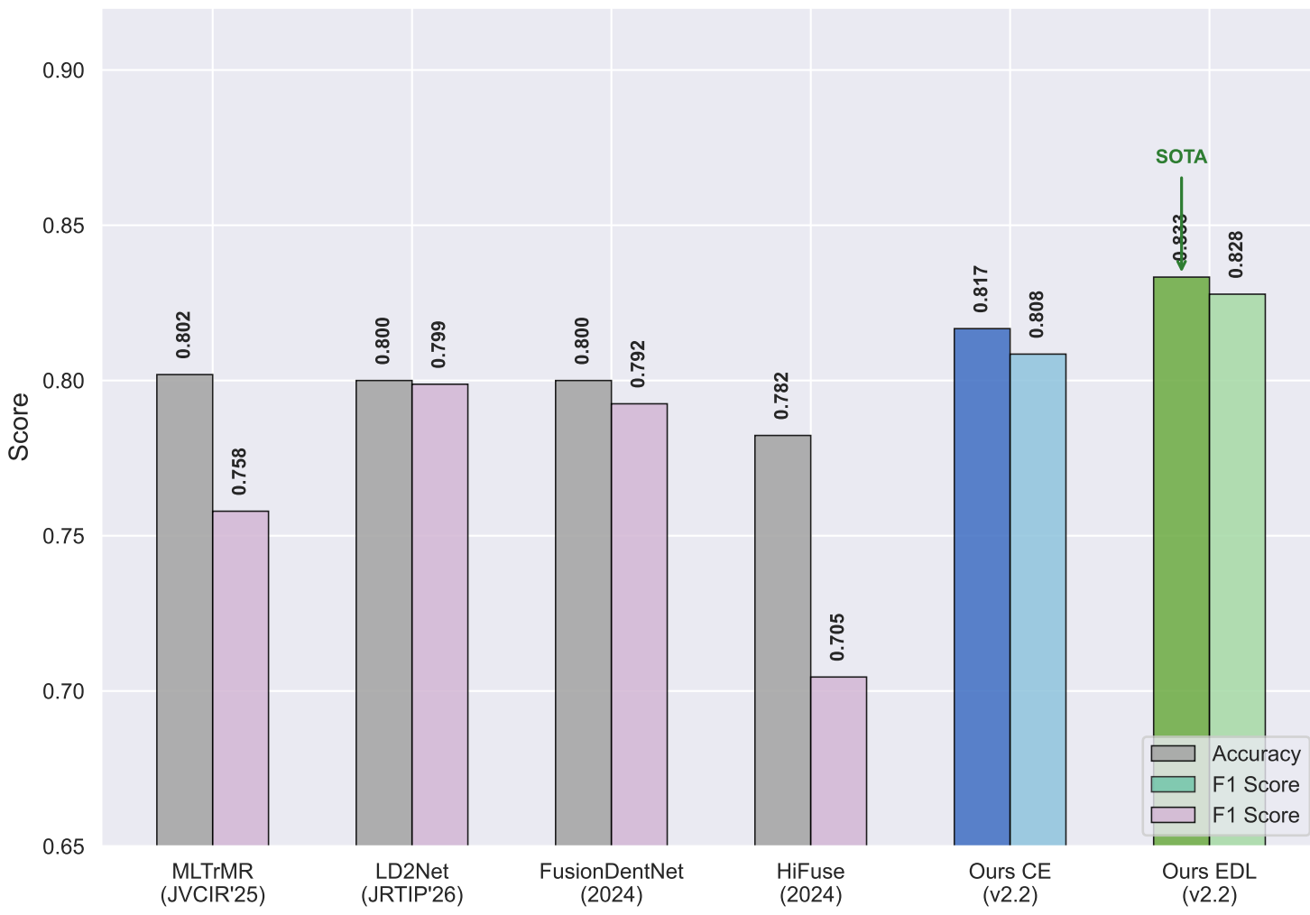
(a) Classification Performance
