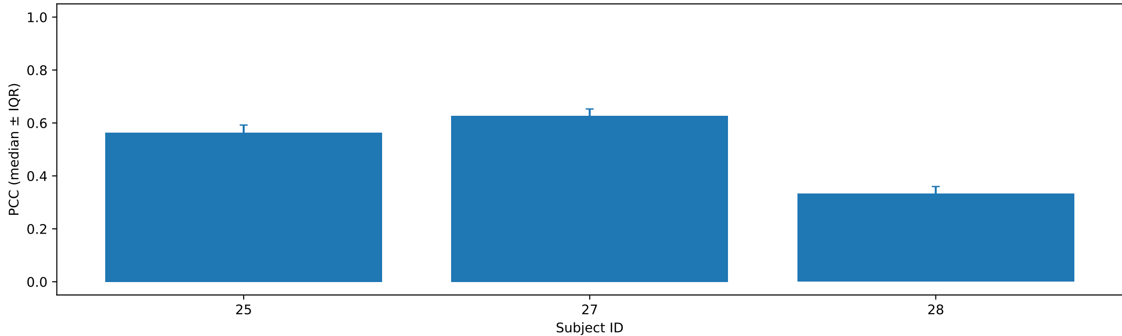
Fig.3 Subject-wise PCC (Median with IQR)
