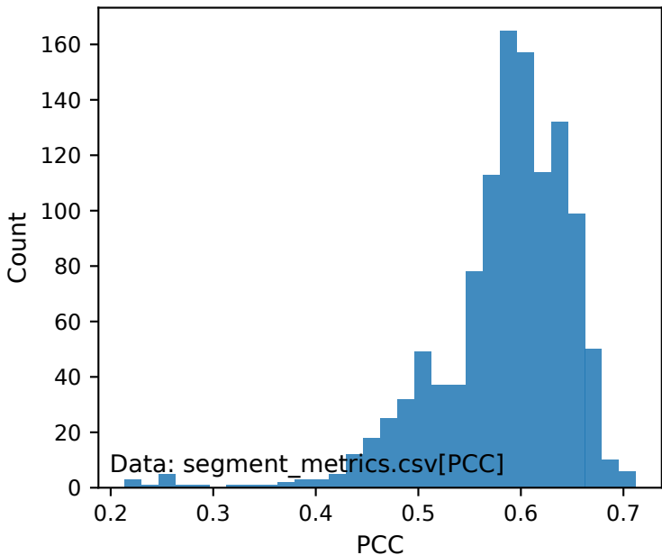
PCC distribution (segment-level)
