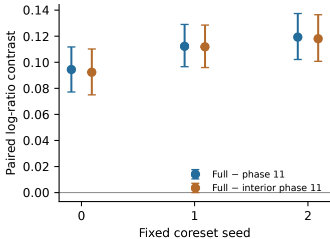
(b) Full-grid contrasts (reference retains boundary)
