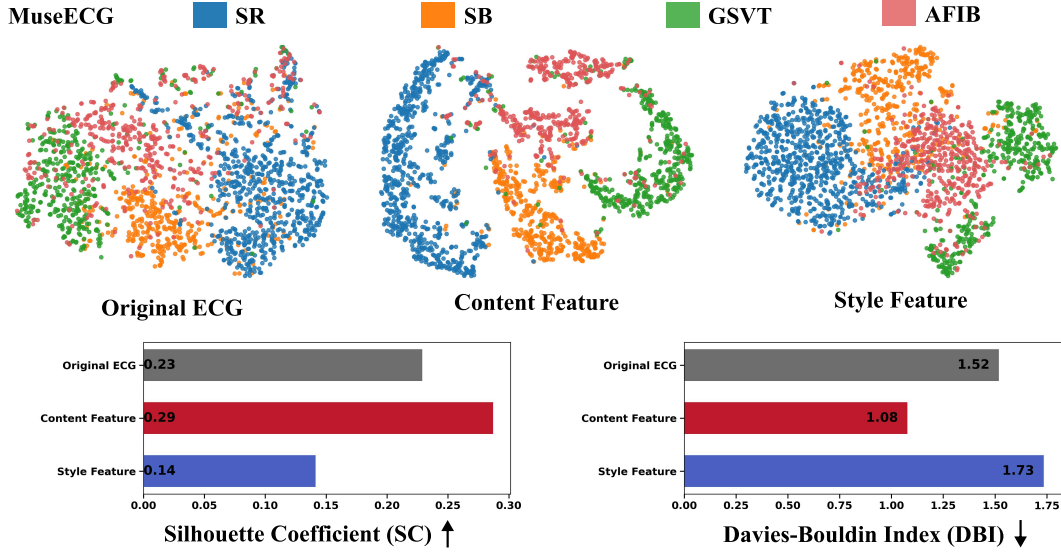
Fig. Appendix 27: Visualization of feature separation on the MuseECG dataset
