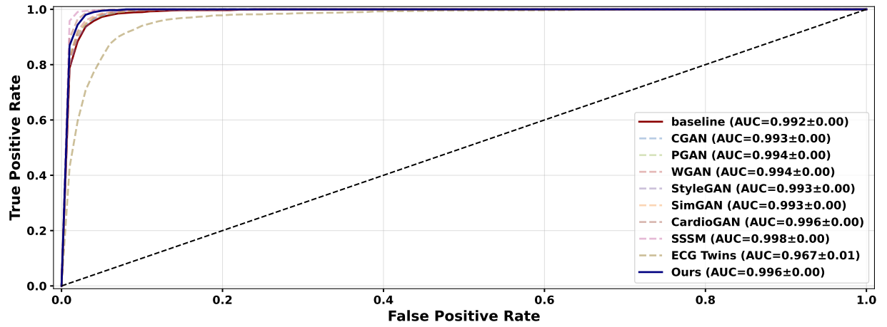
Fig. Appendix 16: ROC Curve – MedalCare-XL (Class: fam)
