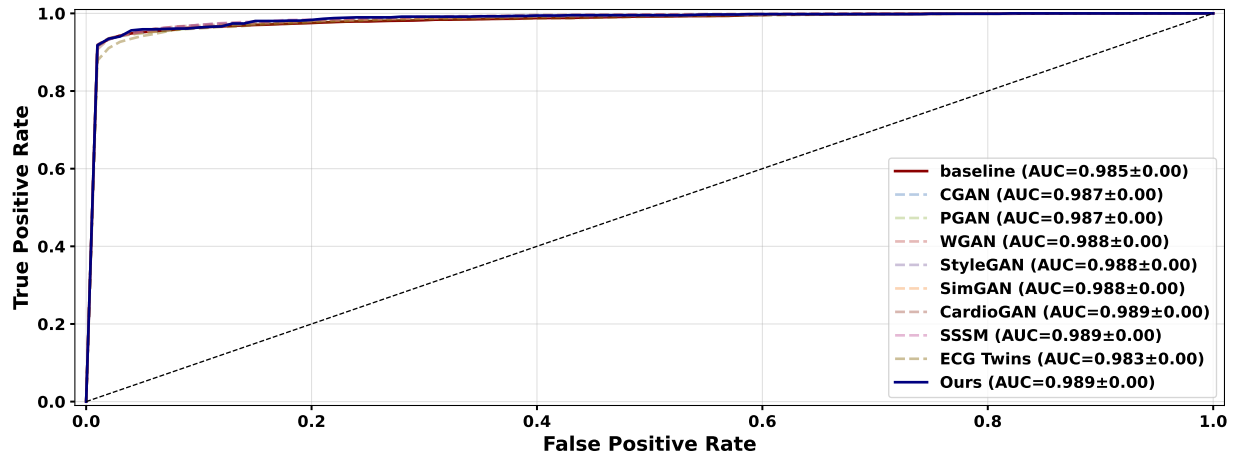
Fig. Appendix 6: ROC Curve – MuseECG (Class: SR)
