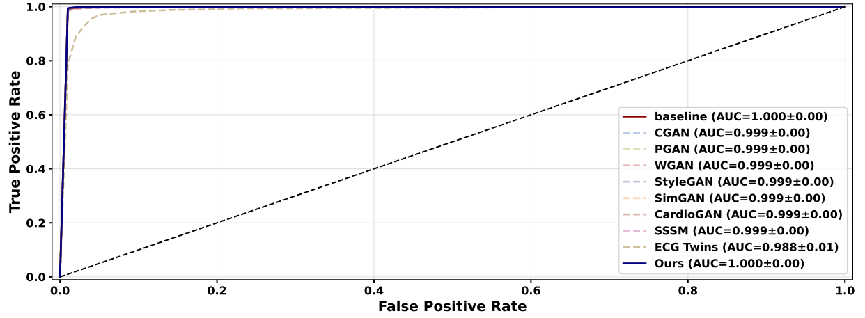
Fig. Appendix 14: ROC Curve – MedalCare-XL (Class: lae)
