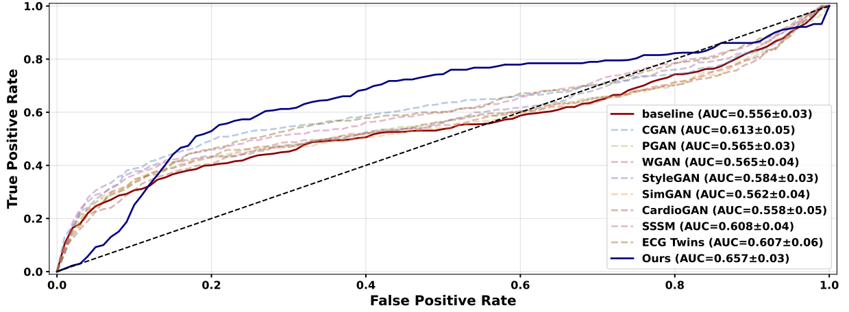
Fig. Appendix 24: ROC Curve – PTB (Class: CD)
