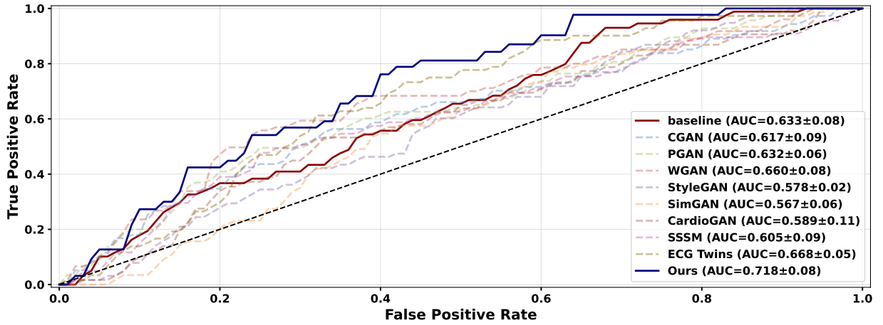
Fig. Appendix 25: ROC Curve – PTB (Class: HYP)
