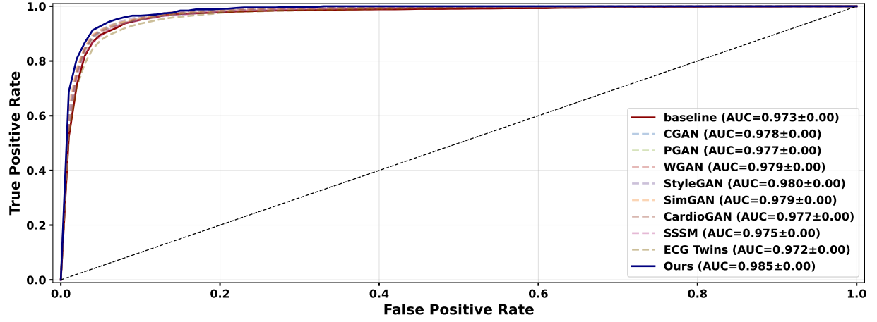
Fig. Appendix 9: ROC Curve – MuseECG (Class: AFIB)
