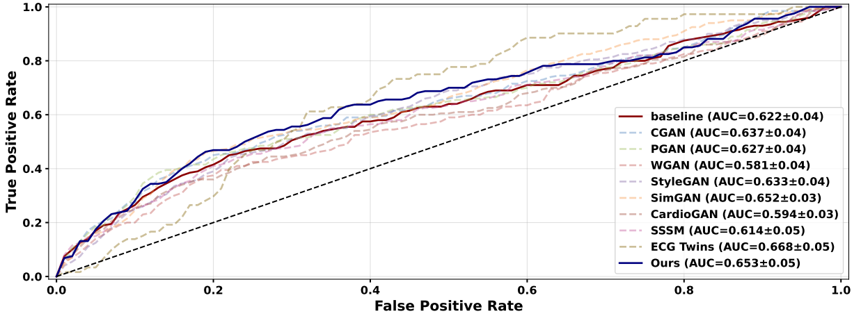
Fig. Appendix 5: ROC Curve – PTB-XL (Class: HYP)
