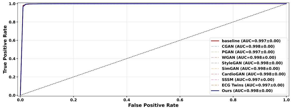
Fig. Appendix 7: ROC Curve – MuseECG (Class: SB)
