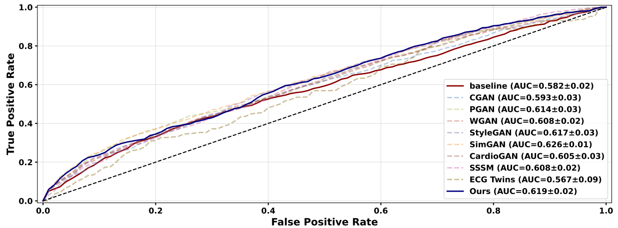
Fig. Appendix 3: ROC Curve – PTB-XL (Class: MI)
