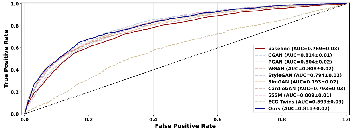
Fig. Appendix 2: ROC Curve – PTB-XL (Class: STTC)
