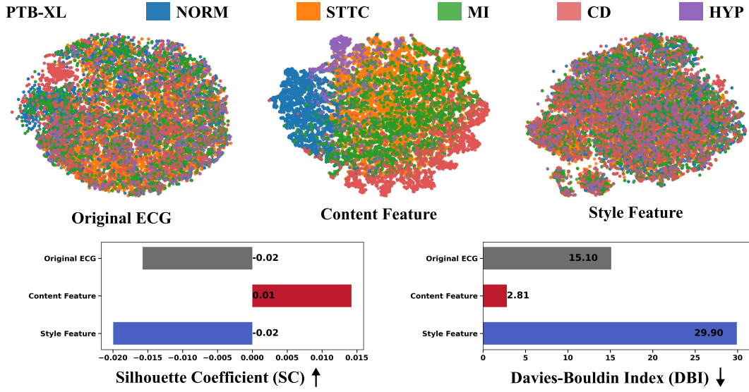
Fig. Appendix 26: Visualization of feature separation on the PTB-XL dataset
