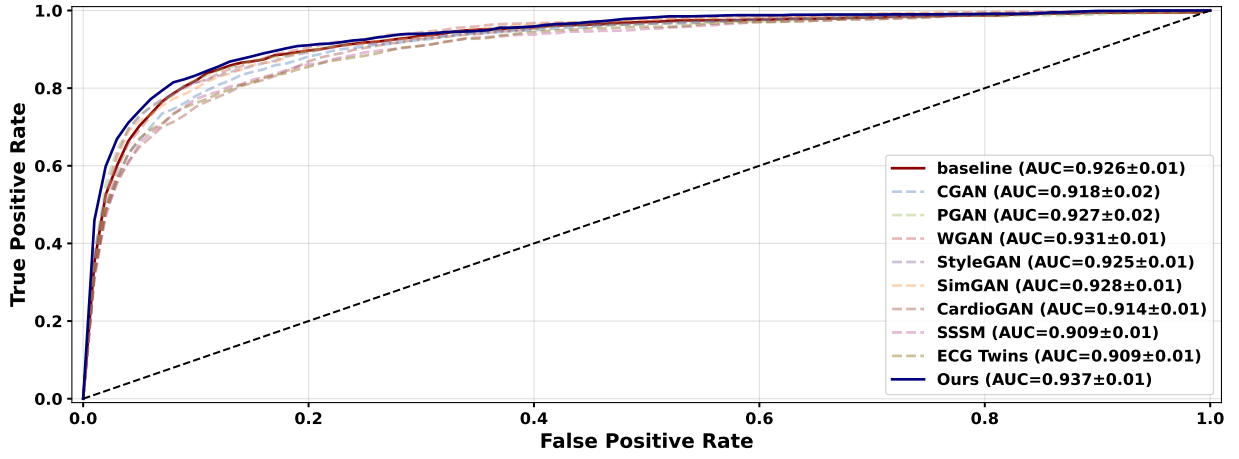
Fig. Appendix 19: ROC Curve – CinC 2017 (Class: A)
