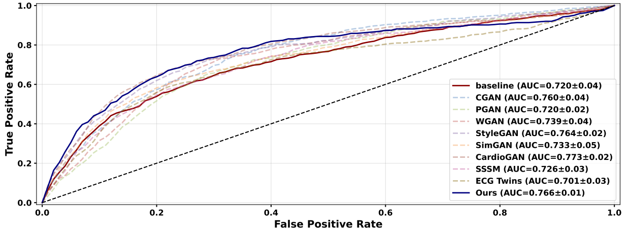
Fig. Appendix 21: ROC Curve – PTB (Class: NORM)
