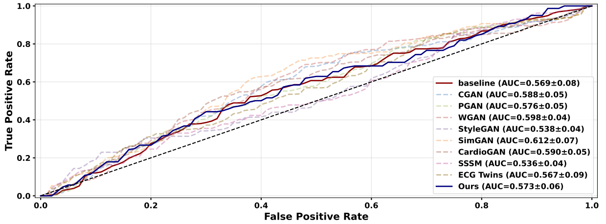
Fig. Appendix 23: ROC Curve – PTB (Class: MI)
