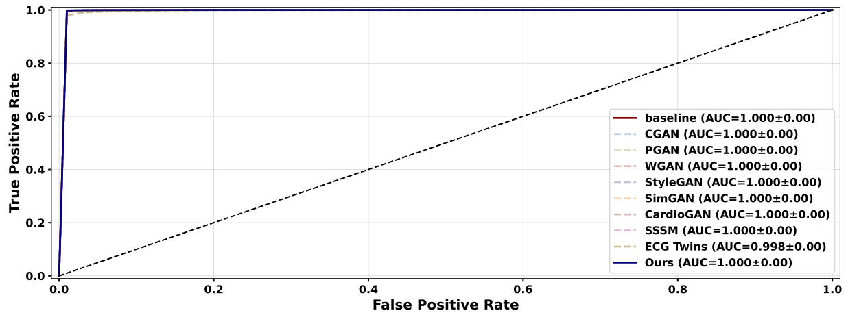
Fig. Appendix 12: ROC Curve – MedalCare-XL (Class: mi)
