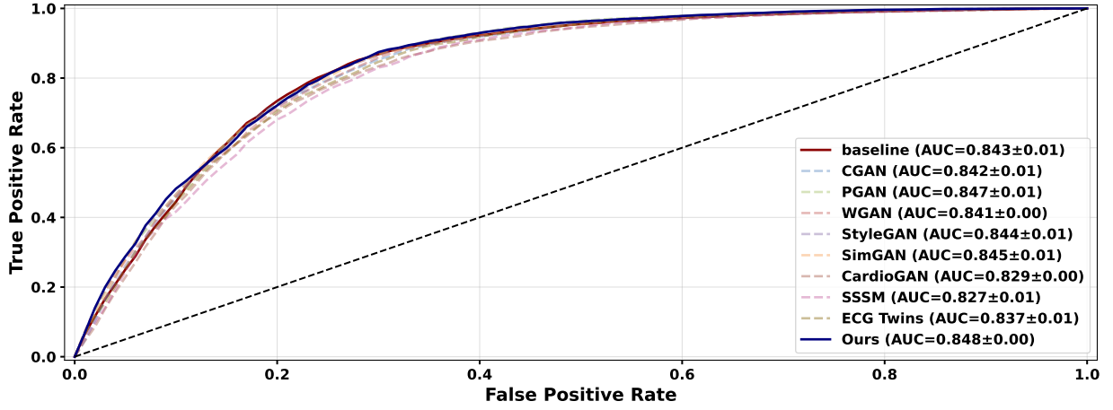
Fig. Appendix 18: ROC Curve – CinC 2017 (Class: N)
