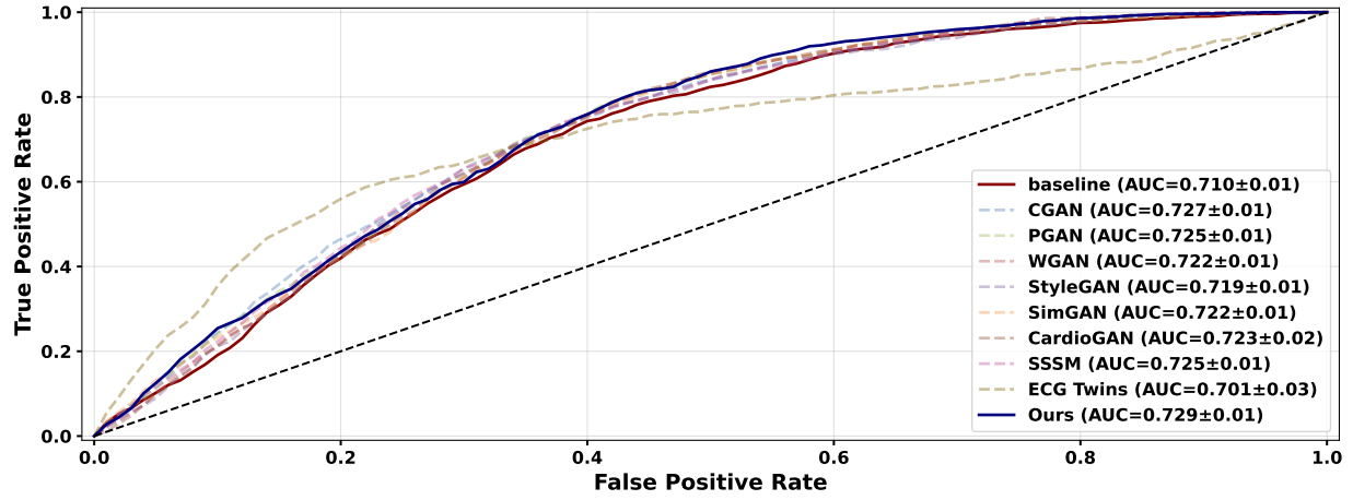
Fig. Appendix 1: ROC Curve – PTB-XL (Class: NORM)
