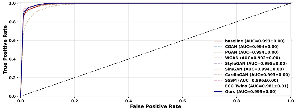
Fig. Appendix 10: ROC Curve – MedalCare-XL (Class: sinus)
