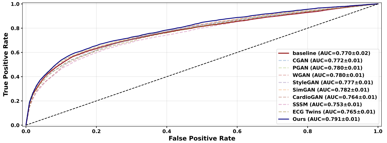
Fig. Appendix 20: ROC Curve – CinC 2017 (Class: O)
