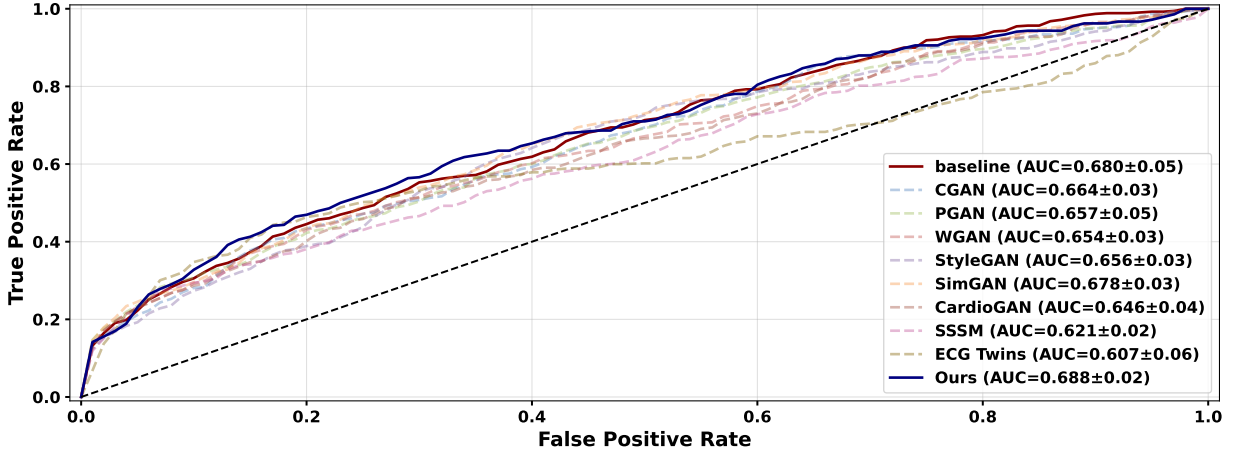
Fig. Appendix 4: ROC Curve – PTB-XL (Class: CD)
