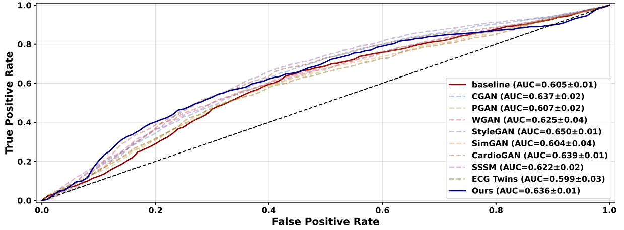
Fig. Appendix 22: ROC Curve – PTB (Class: STTC)
