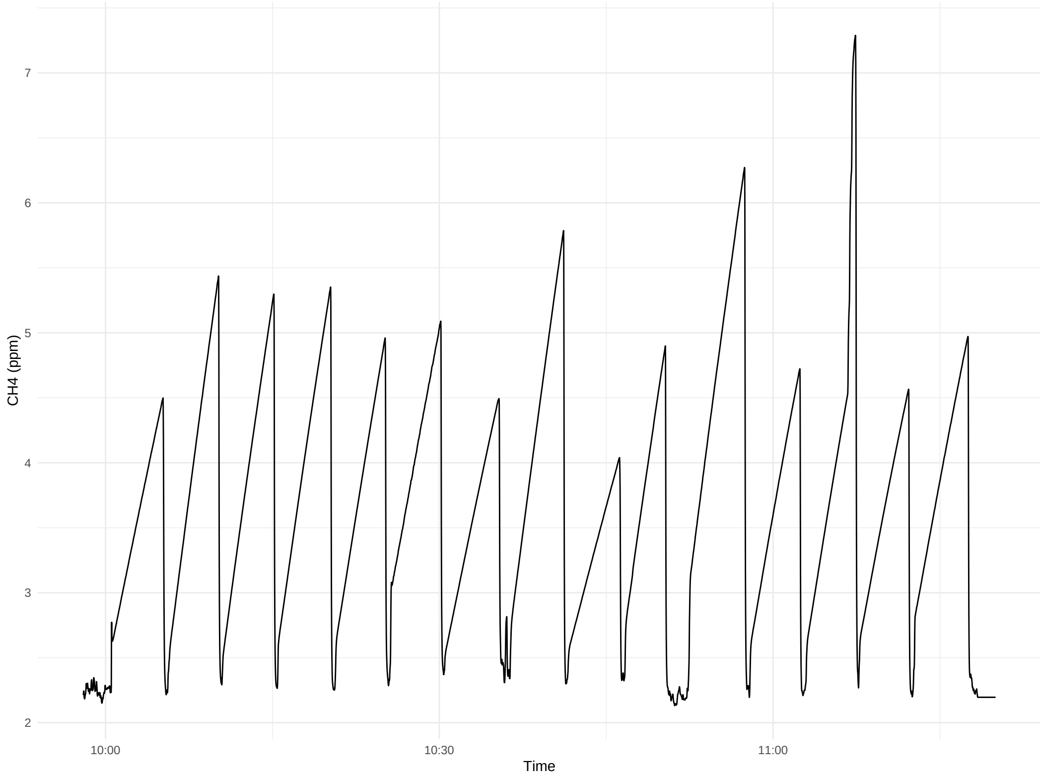
CH4 Over Time – 2025-08-04
