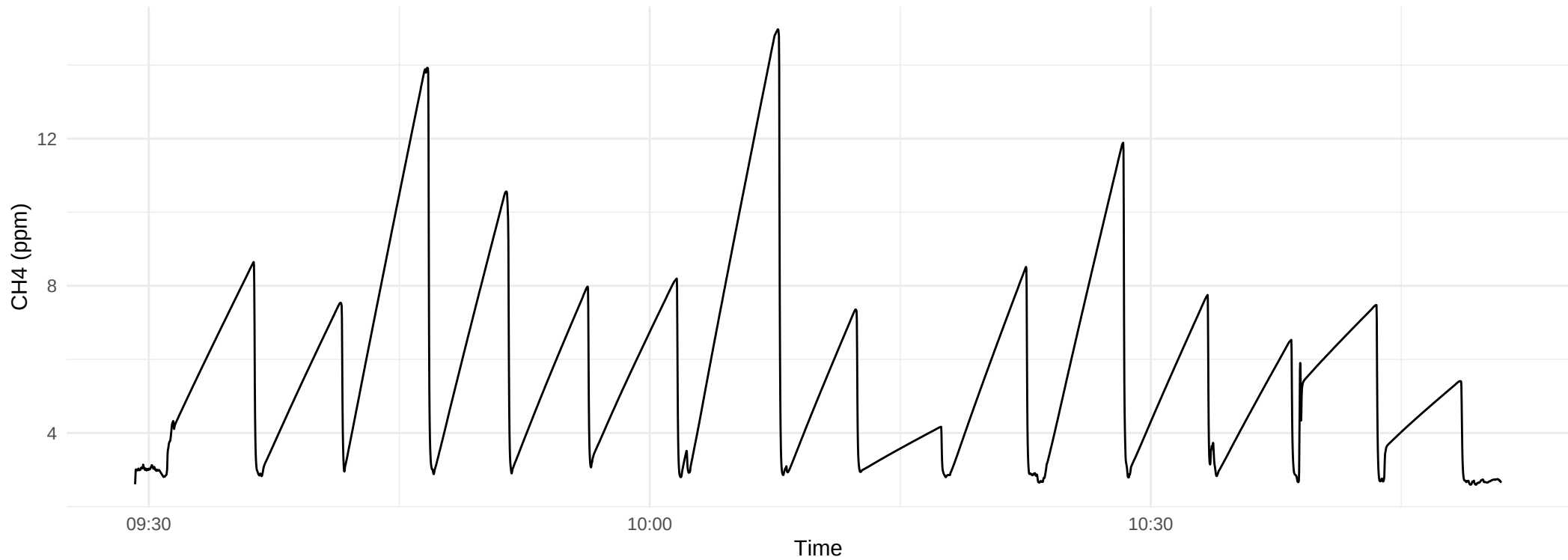
CH4 Over Time – 2025-06-27
