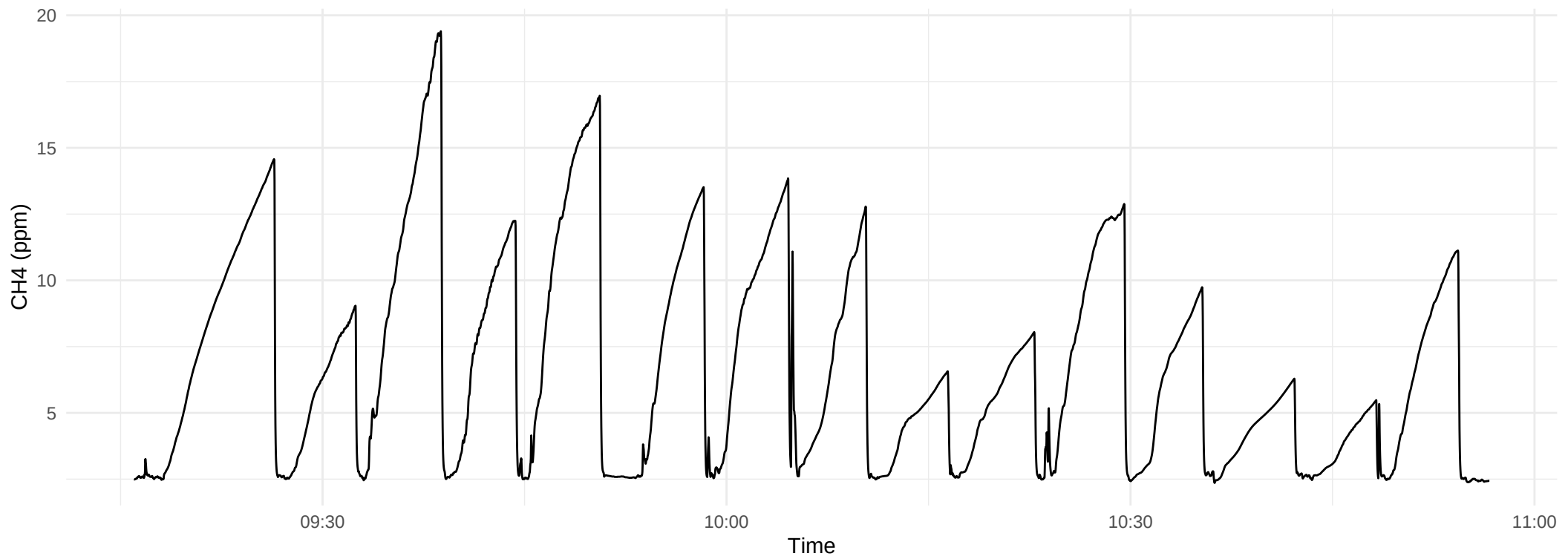
CH4 Over Time – 2025-06-09
