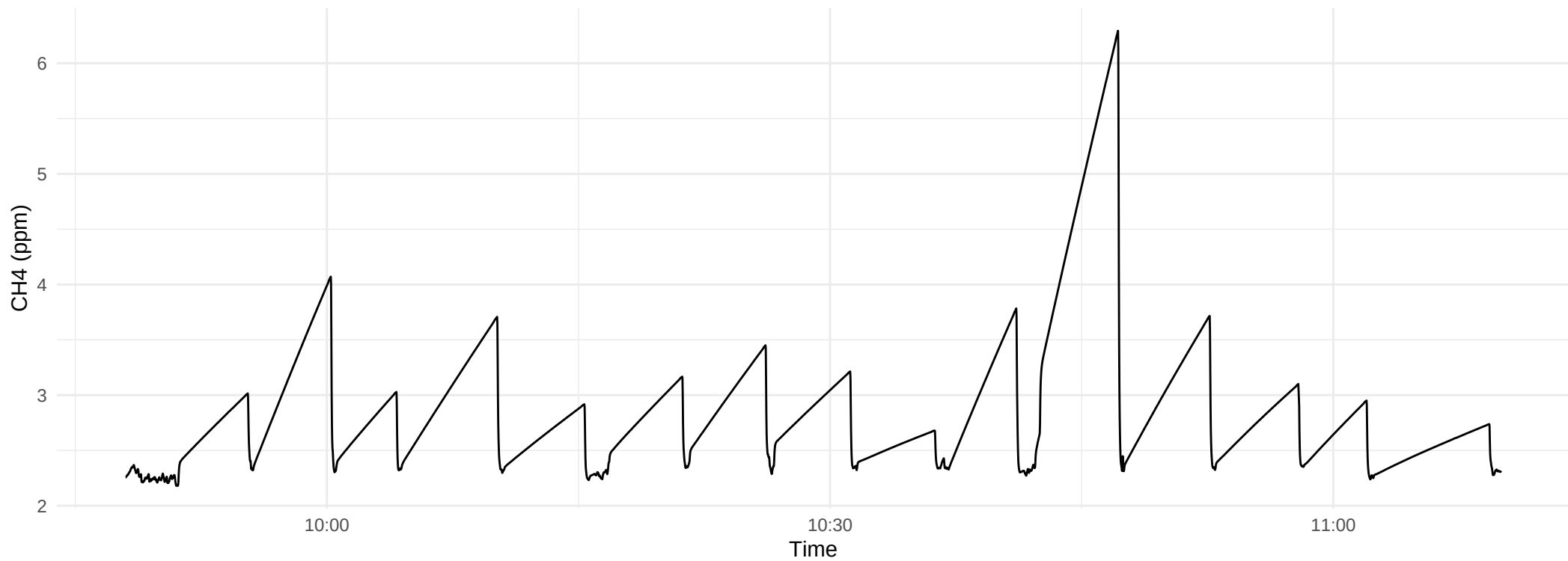
CH4 Over Time – 2025-07-11
