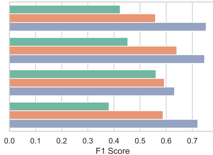
ML Efficiency
