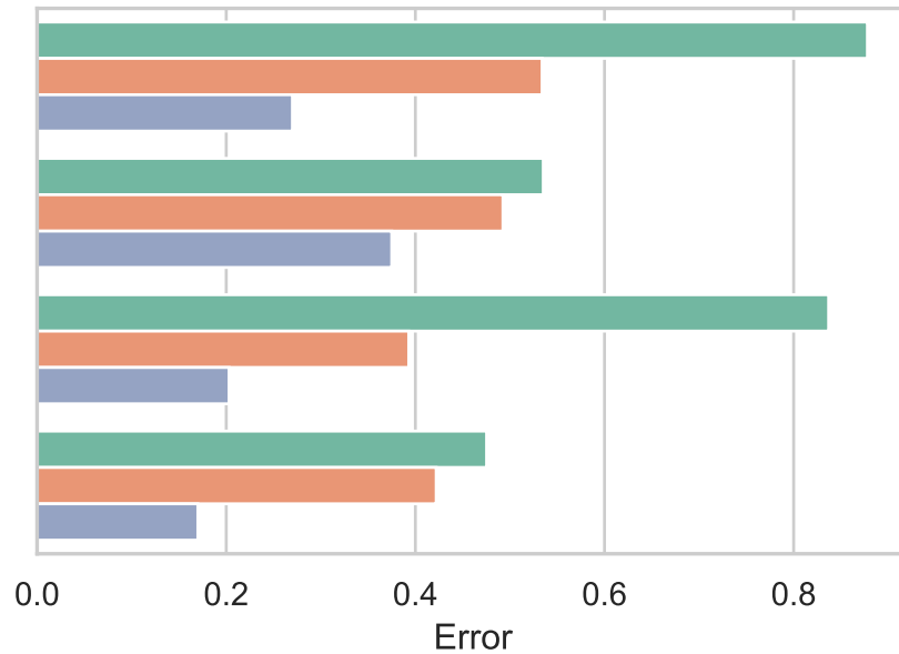
Fidelity Error
