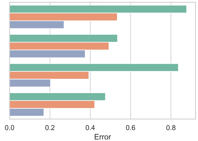
Fidelity Error
