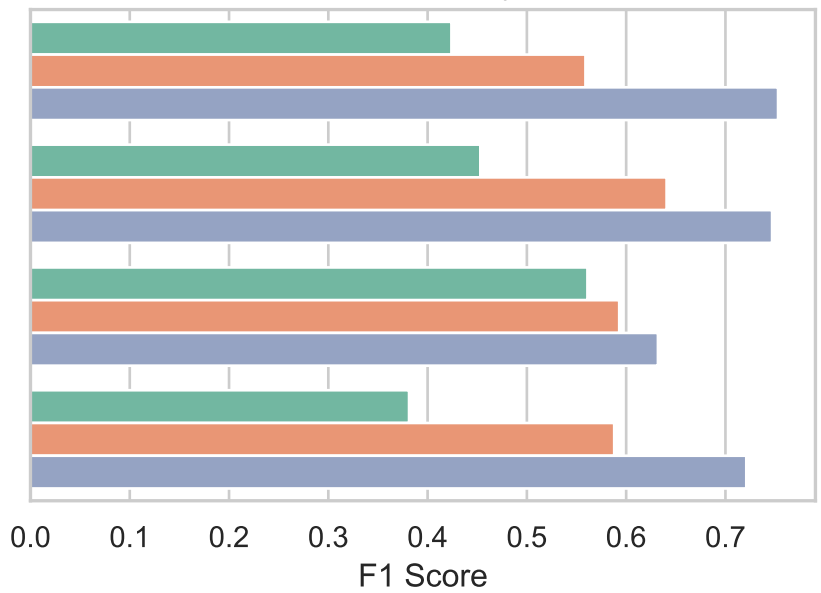
ML Efficiency
