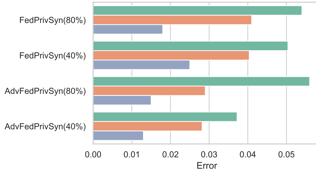
Query Error
