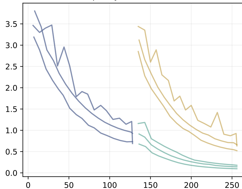
On-policy OPD reverse KL
