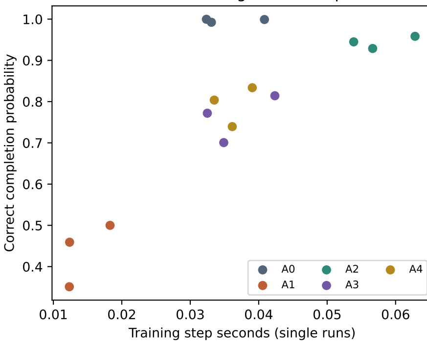
Observed learning vs CPU step cost
