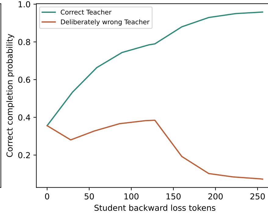
Failure control: Teacher error transfer
