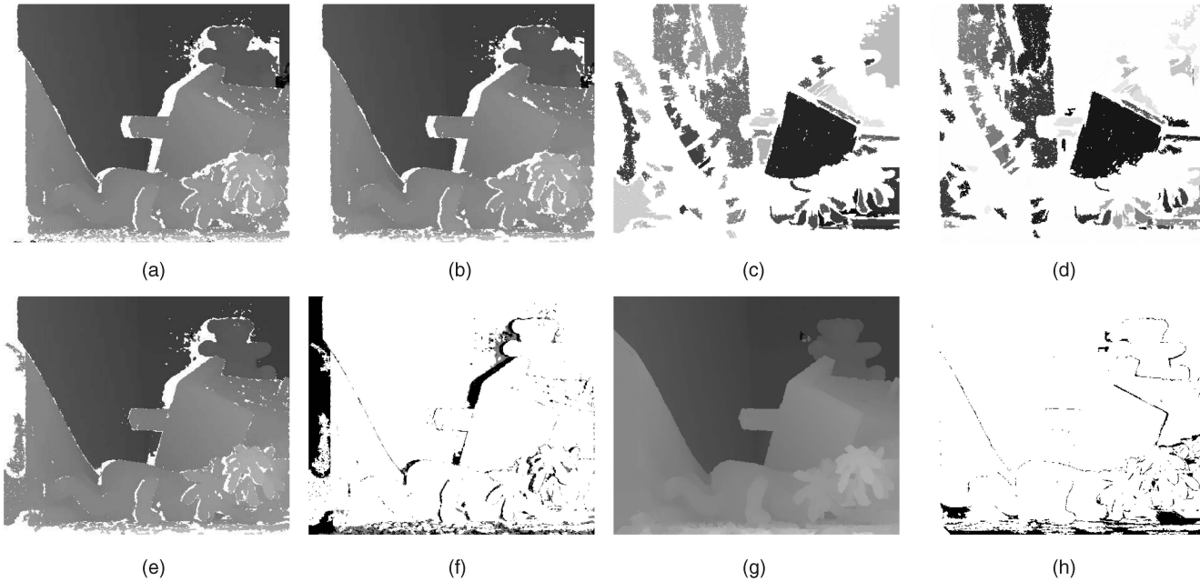
Fig. 13. Demonstration of the effect of the proposed postprocessing steps on the Teddy images. (a) Result after basic SGM. (b) Result after peak filtering. (c) Low textured segments. (d) Disparity segments. (e) Intensity Consistent Sel. (f) Occlusions (black) and mismatches (gray). (g) Result after interpolation. (h) Errors against ground truth.
