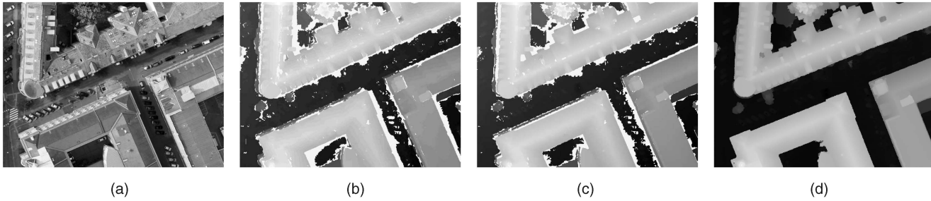
Fig. 14. SGM matching results from aerial UltraCam images of Graz. The input image block is a courtesy of Vexcel Imaging Graz. (a) Small part of aerial image. (b) Matching against one image. (c) Matching against six images. (d) Orthographic reprojection.
