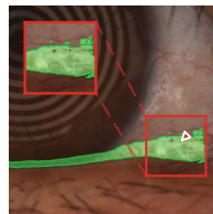
SAM2 MSA
