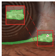
SAM2 Base
