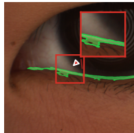
Swin-UNETR
